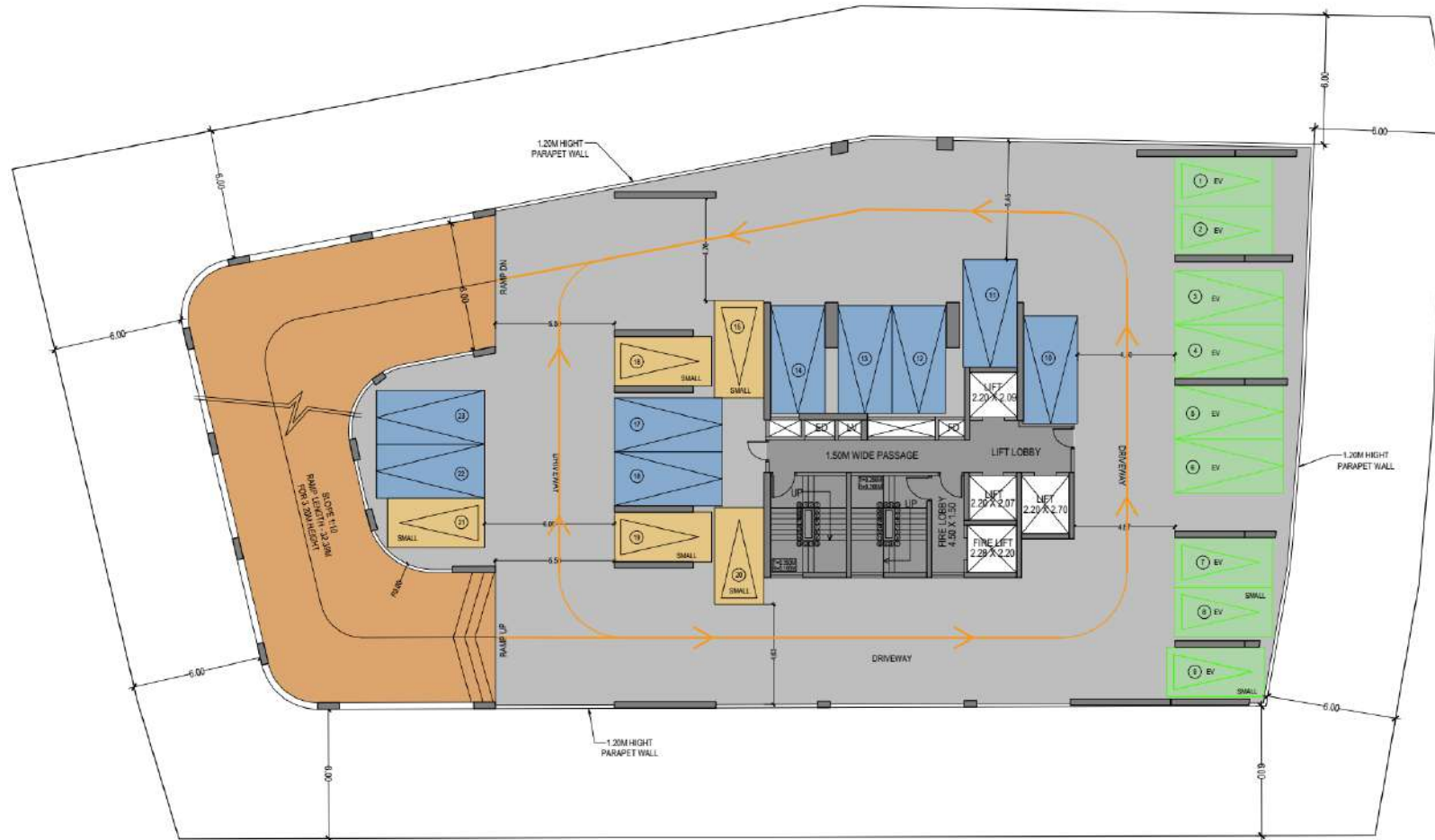
2ND TO 5TH PODIUM FLOOR PLAN
