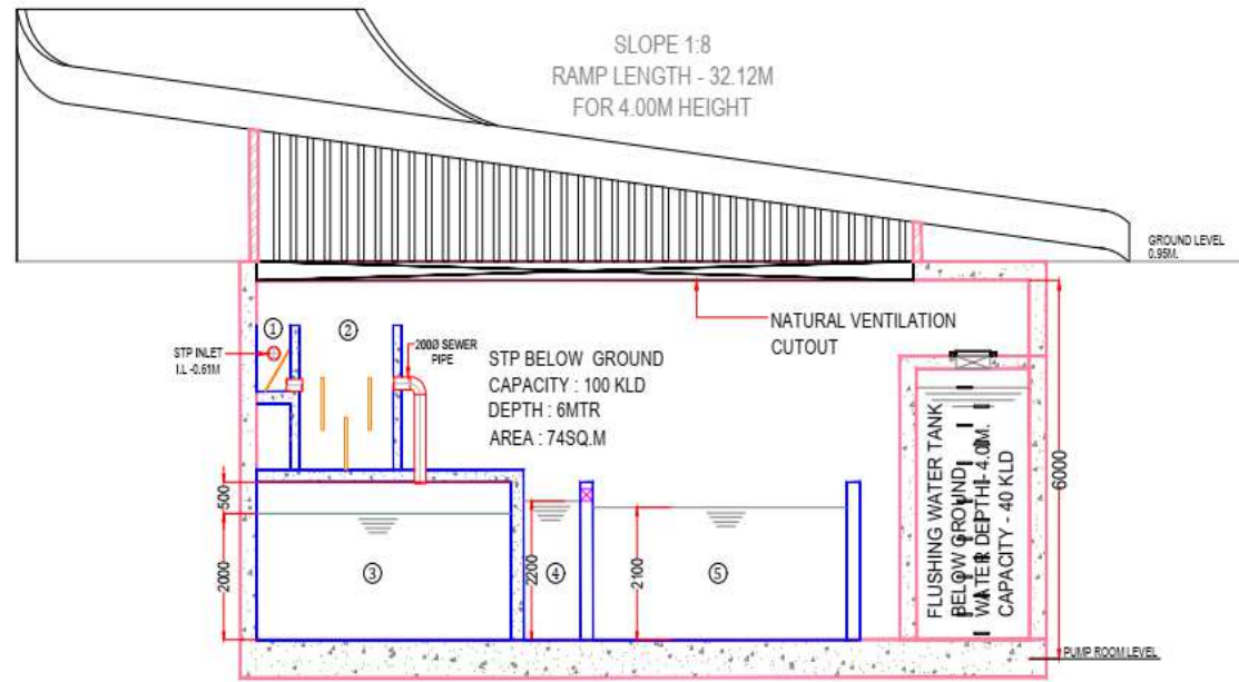
SECTION B-B (STP) SCALE 1:100
